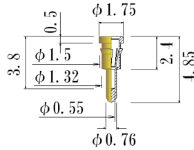
Acceptable plug: \phi 0.60 \sim \phi 0.40 JS0041-1L-GG
