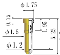
Acceptable plug: \phi 0.60 \sim \phi 0.40 JS0062-L-GG
