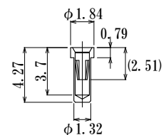
JS0020-GG-856 (J-856contact, Low force, Six fingers) 受注生産品
