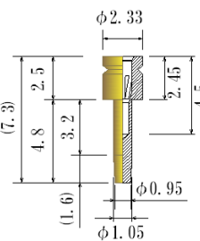
NSB11V-GG
