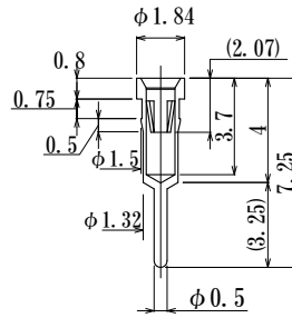
J0010-GG-634 (J-634contact, High force)
