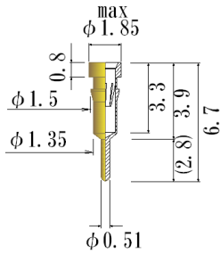
Acceptable plug: \phi 0.60 \sim \phi 0.40 J0010-L-GG
