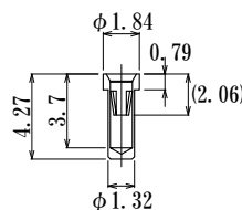
JS0020-GG-ST (JV11contact, value type)
