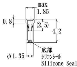
JSP0020-GG-TF
