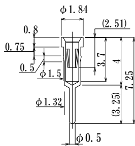
J0010-GG-ST (Value type)
