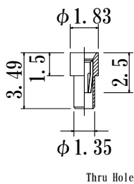
JSP0021-GG
