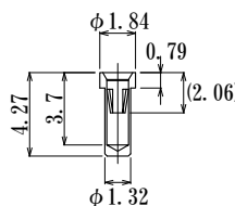
JS0020-GG-634 (J-634contact, High force)
