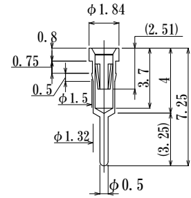
J0010-GG-856 (J-856contact, Low force, Six fingers) 受注生産品
