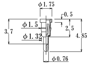
Acceptable plug: \phi 0.60 \sim \phi 0.40 JS0041B-GG
