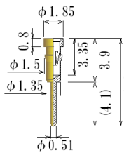
J0010-GG-ST (Value type)
