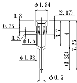
J0010-GG-JV11 (JV11contact, value type)
