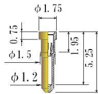
Acceptable plug: \phi 0.60 \sim \phi 0.40 JS0062-L-GG
